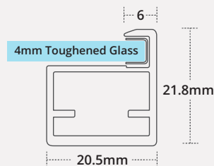
Profile Dimensions 1:1 Scale
