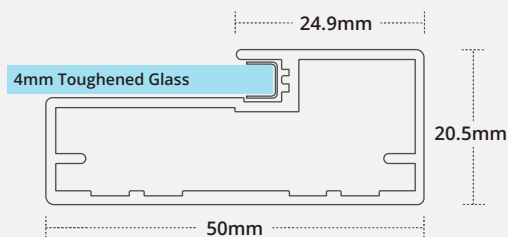
Profile Dimensions 1:1 Scale
