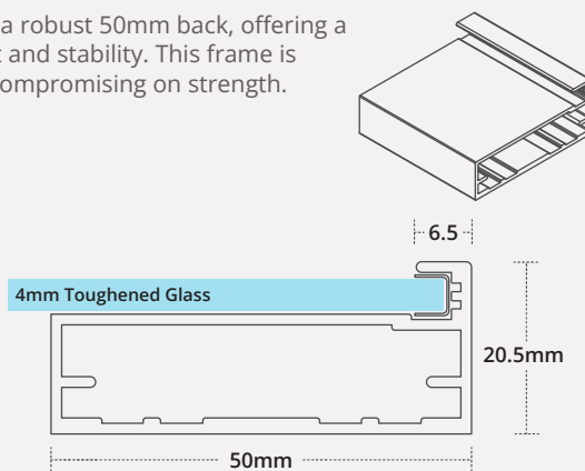
Profile Dimensions 1:1 Scale
