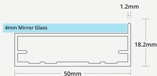
Profile Dimensions 1:1 Scale
