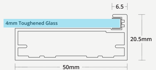
Profile Dimensions 1:1 Scale
