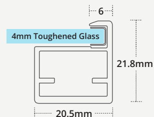
Profile Dimensions 1:1 Scale
